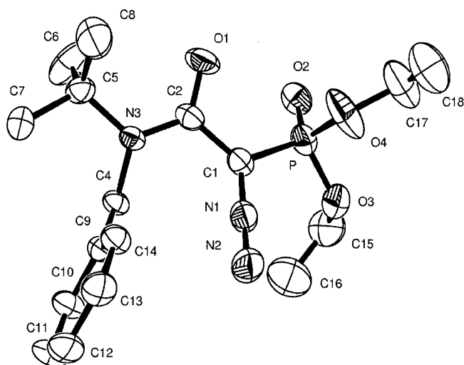
Figure 2. Crystal structure of the diazo 4l ; selected bond lengths [Å] and angles [°]: P–C(1) 1.778(2), O(1)–C(2) 1.225(3), N(1)–N(2) 1.125(3), N(1)–C(1) 1.311(3), C(1)–C(2) 1.488(3), C(2)–N(3) 1.359(3), O(2)–P–C(1) 118.9(3), N(1)–C(1)–P 116.07(17), C(2)–C(1)–P 121.29(15), O(1)–C(2)–N(3) 123.6(2), O(1)–C(2)–C(1) 115.92(19), N(3)–C(2)–C(1) 120.50(18), C(2)–N(3)–C(4) 120.56(17), C(2)–N(3)–C(5) 118.93(17).
